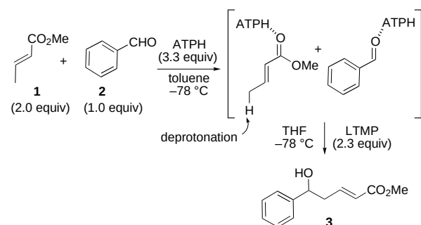
Scheme 1. Crossed-aldol condensation of methyl crotonate ( 1 ) with benzaldehyde ( 2 ) using ATPH and LTMP.
